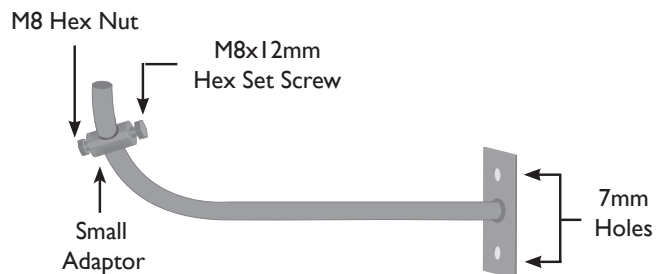
ZINC PLATED ECONOMY J-BRACKET
