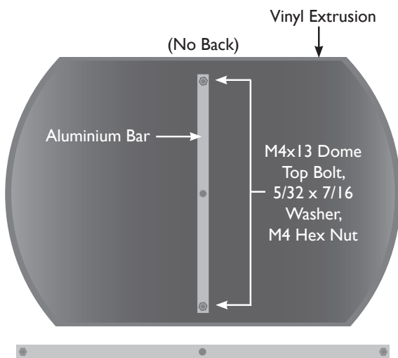
REAR VIEW
