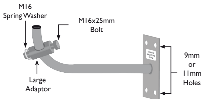
ZINC PLATED HEAVY DUTY J-BRACKET
